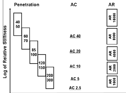
Fig. 15. Comparison of Penetration and Viscosity bitumen grades.
