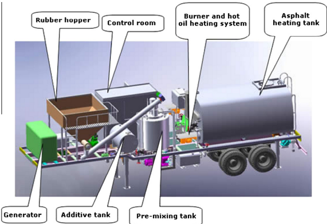
Fig. 12. Example of mobile Mixing unit for Asphalt-Rubber, adapted from [34].
