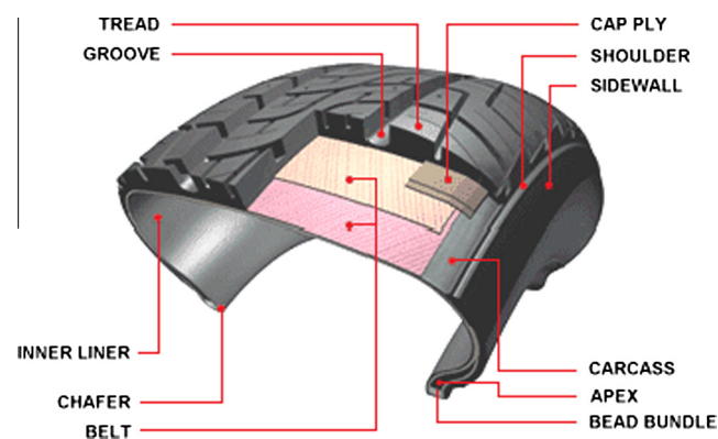
Fig. 2. Tyre structure, adapted from [7].
